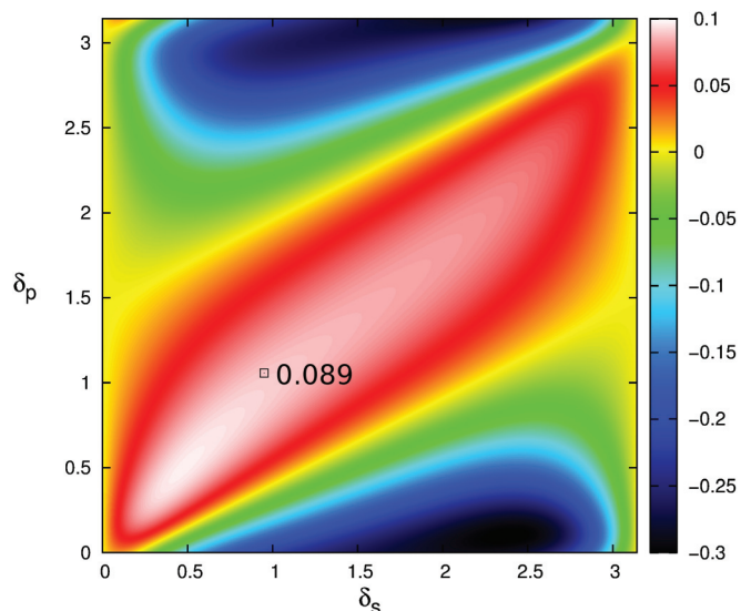
FIG. 2. (Color online) The dependence of the spin Hall angle, given by Eq. (28), on \delta_s \equiv \delta_{1/2}^s and \delta_p \equiv \frac{1}{3}(\delta_{1/2}^p + 2\delta_{3/2}^p) is shown for the relaxed geometry together with the corresponding value of \alpha from Table III.
